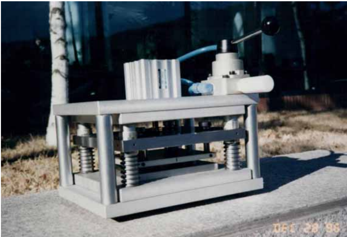
GUIDE HOLE PUNCHING MACHINE
